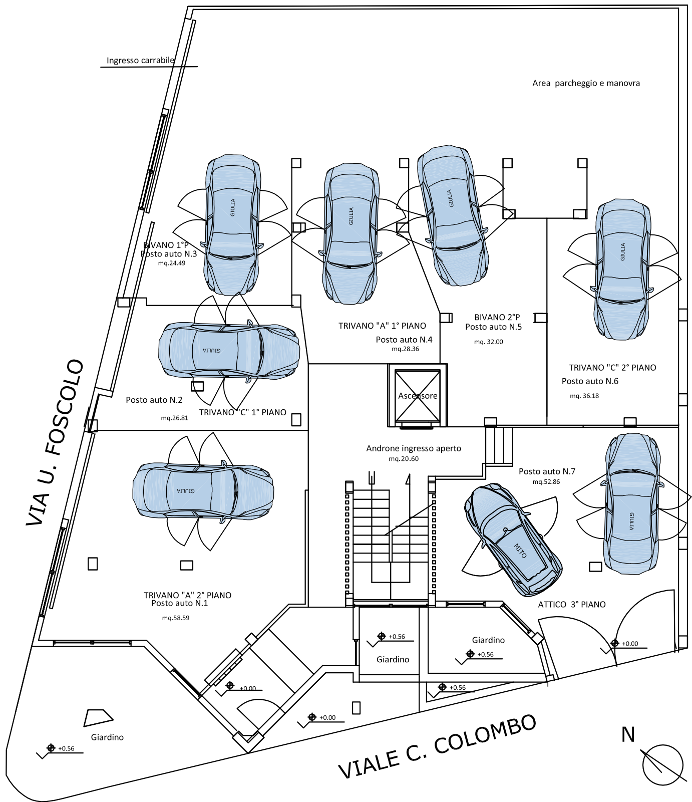
PIANO PILOTIS SC. 1:100
